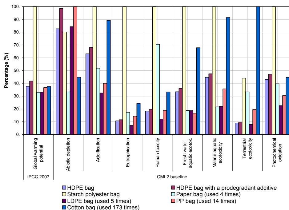
Figure 6.5 The results of the impact assessment when the IPCC 2007 and CML 2 baseline methods were used.
