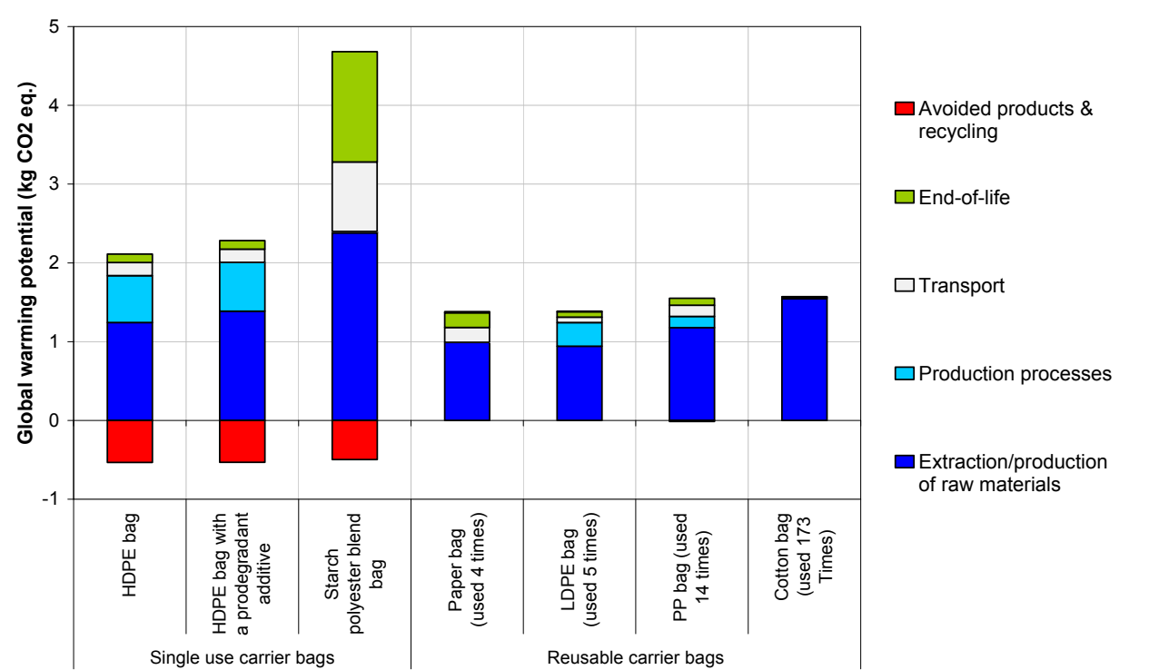
Figure 5.2 The global warming potential impacts of each type of carrier bag assuming each is reused to outperform a conventional HDPE bag with no reuse).
