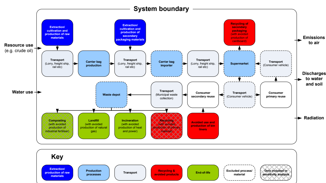
Figure 3.1 System boundaries applied in this study (simplified flow diagram).
